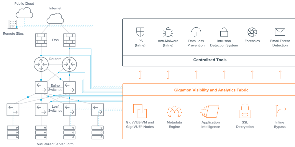
Figure 1: Aggregate traffic to the Gigamon Visibility Platform
